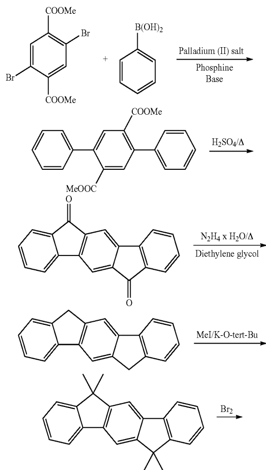
Synthesis scheme 1: Precursors of indenofluorene derivatives
