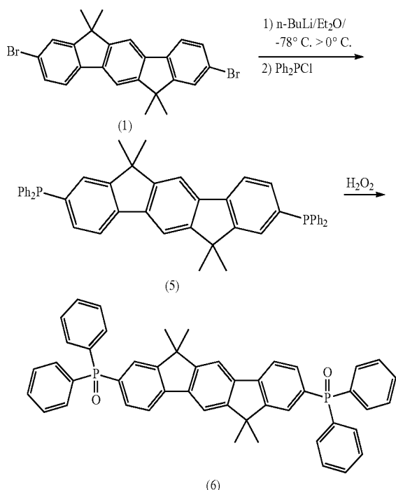
Synthesis scheme 3: Indenofluorene-phosphine compounds
