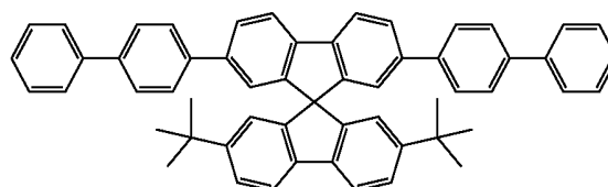
Host H3
