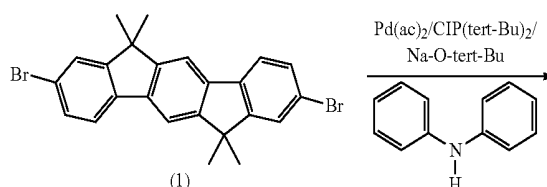
Synthesis scheme 2: Indenofluorene-amine compounds
